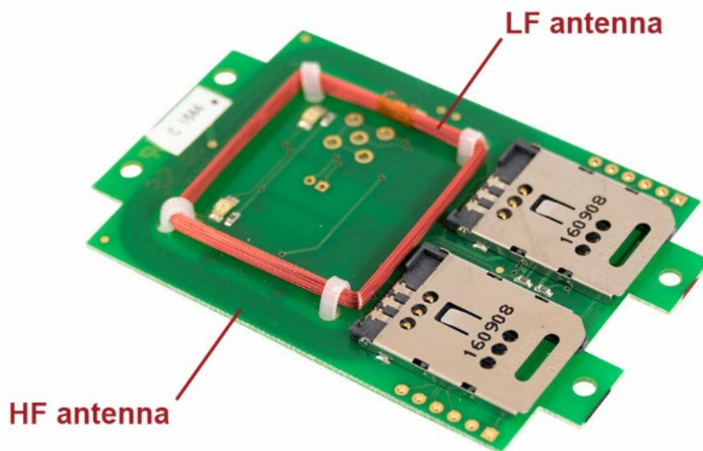
PCB contained in TWN4 MultiTech
